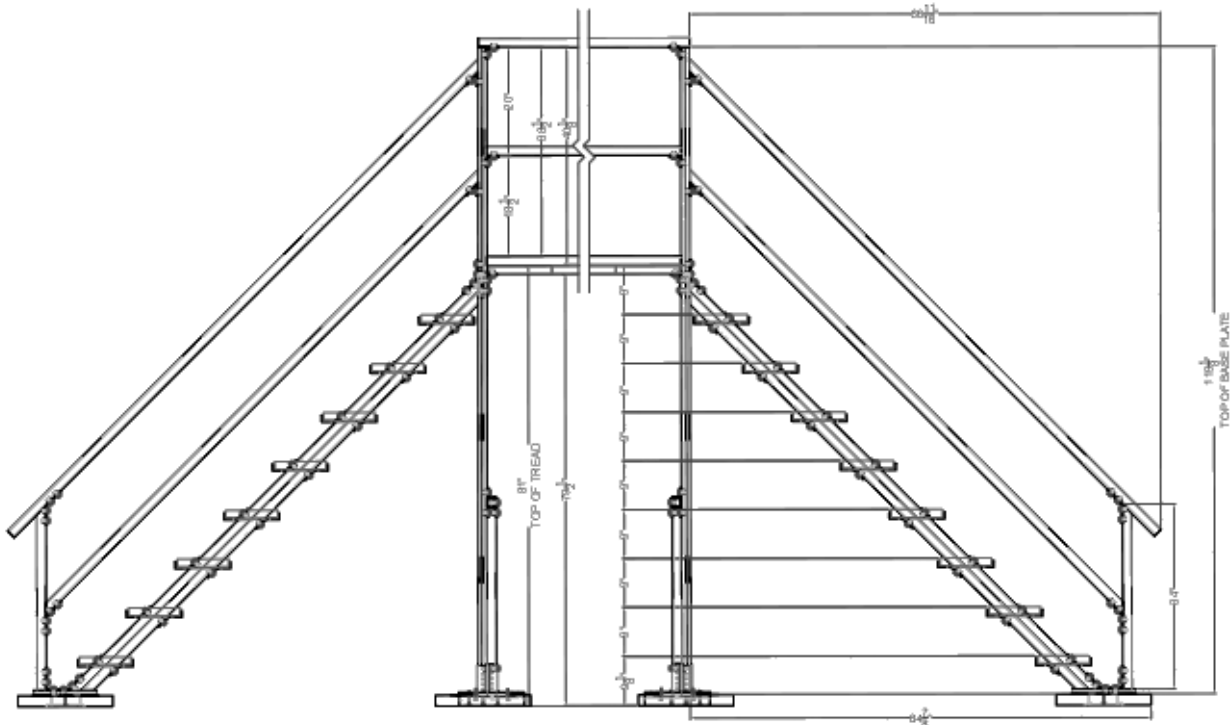
ELEVATION VIEW
