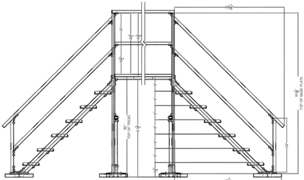
ELEVATION VIEW
