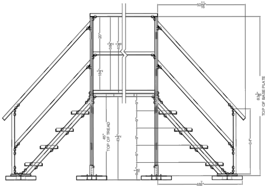
ELEVATION VIEW
