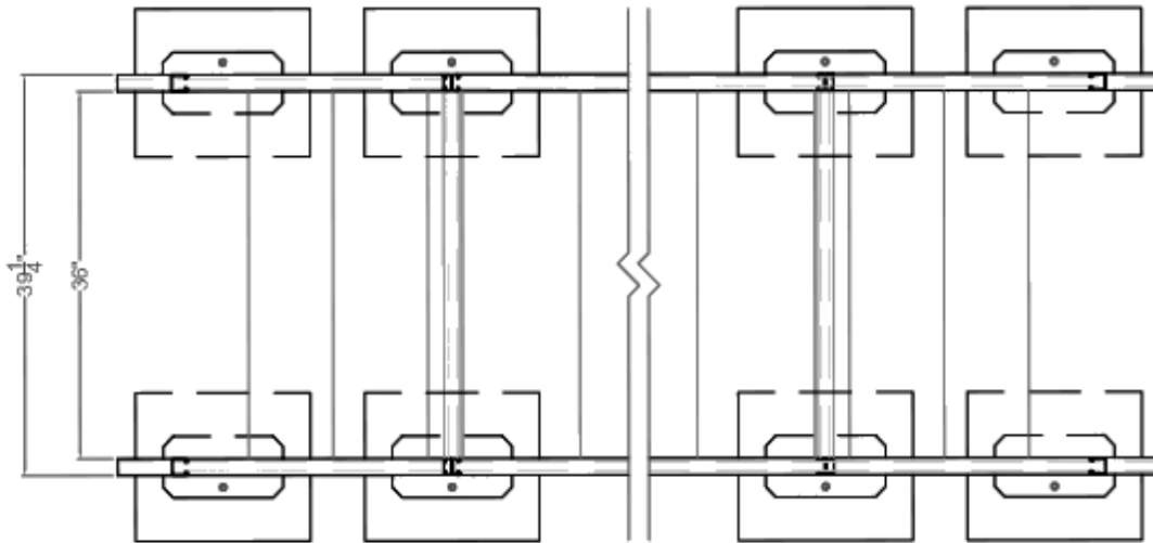
PLAN VIEW
