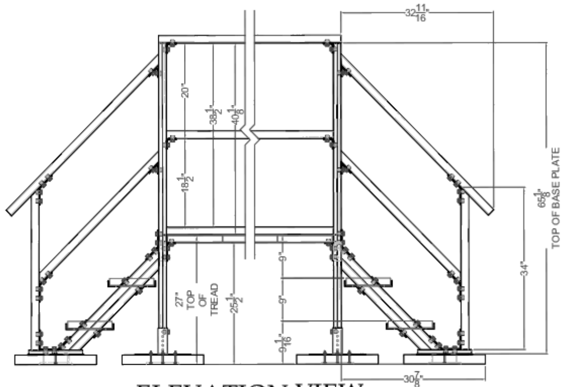
ELEVATION VIEW
