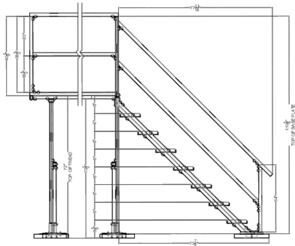
ELEVATION VIEW
