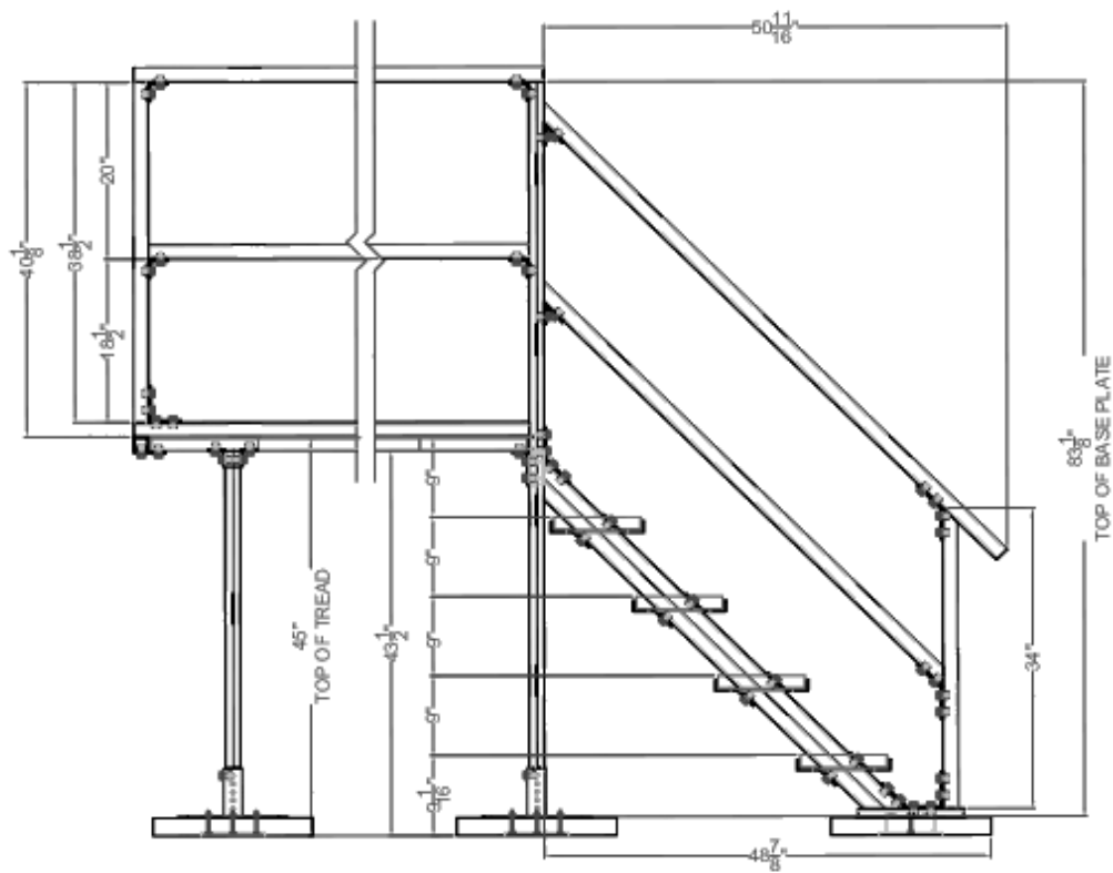
ELEVATION VIEW
