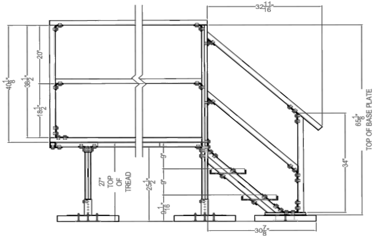
ELEVATION VIEW
