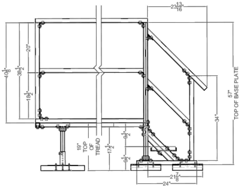
ELEVATION VIEW
